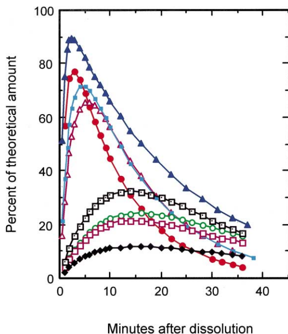
Figure 2. Aziridinium ion formation and decay at pH 7.4 and 37°C for compounds 9 (●), 10 (▲), 11 (△), 12 (■), 16a (○), 16b (□), 17 (▣) and 18 (◆).
